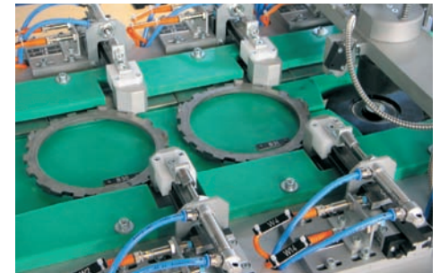
DryLin® 用于汽车行业涡流探伤检测 DryLin® test station for the eddy-current crack test of components for the automobile industry
