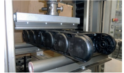
破坏性测试: 计算最大架空长度 break test: calculation of max. unsupported length
